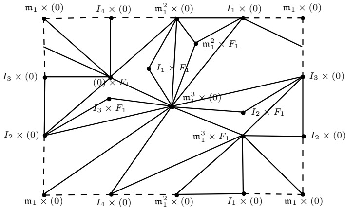
Fig 2.12: Torus embedding of \mathbb{A}\mathbb{G}(R_1 \times F_1) with n_1 = 4, I_1m_1^2 = (0) ,
