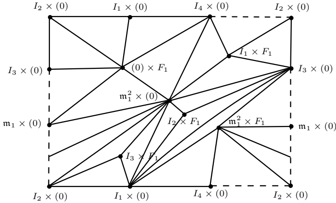
Fig 2.9: Torus embedding of \mathbb{A}\mathbb{G}(R_1 \times F_1) with n_1 = 3 , I_i m_1 \neq (0)
