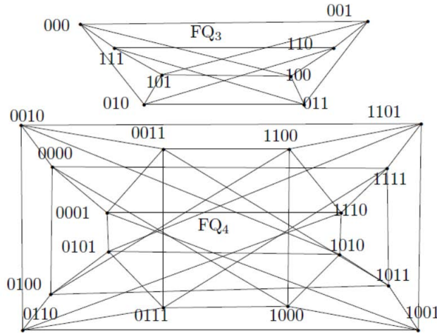
Figure 1. The folded hypercubes FQ_3 and FQ_4
