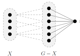
Figure 7. Construction of G_X in Lemma 7.
