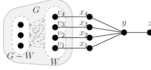
Figure 5. The construction of G_u from G in Lemma 5.
