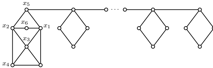
Figure 3. Graph G''_\ell
