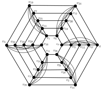
Figure 3. Ordering of vertices K_5 \square C_6 as described in Lemma 7
