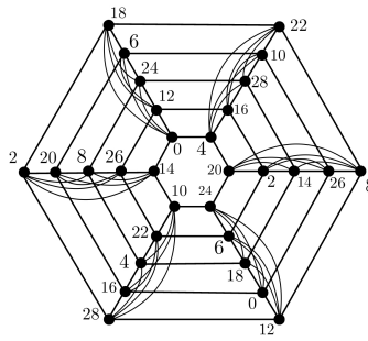
Figure 4. The antipodal coloring of K_5 \square C_6 as described in Theorem 5 with span 28.
